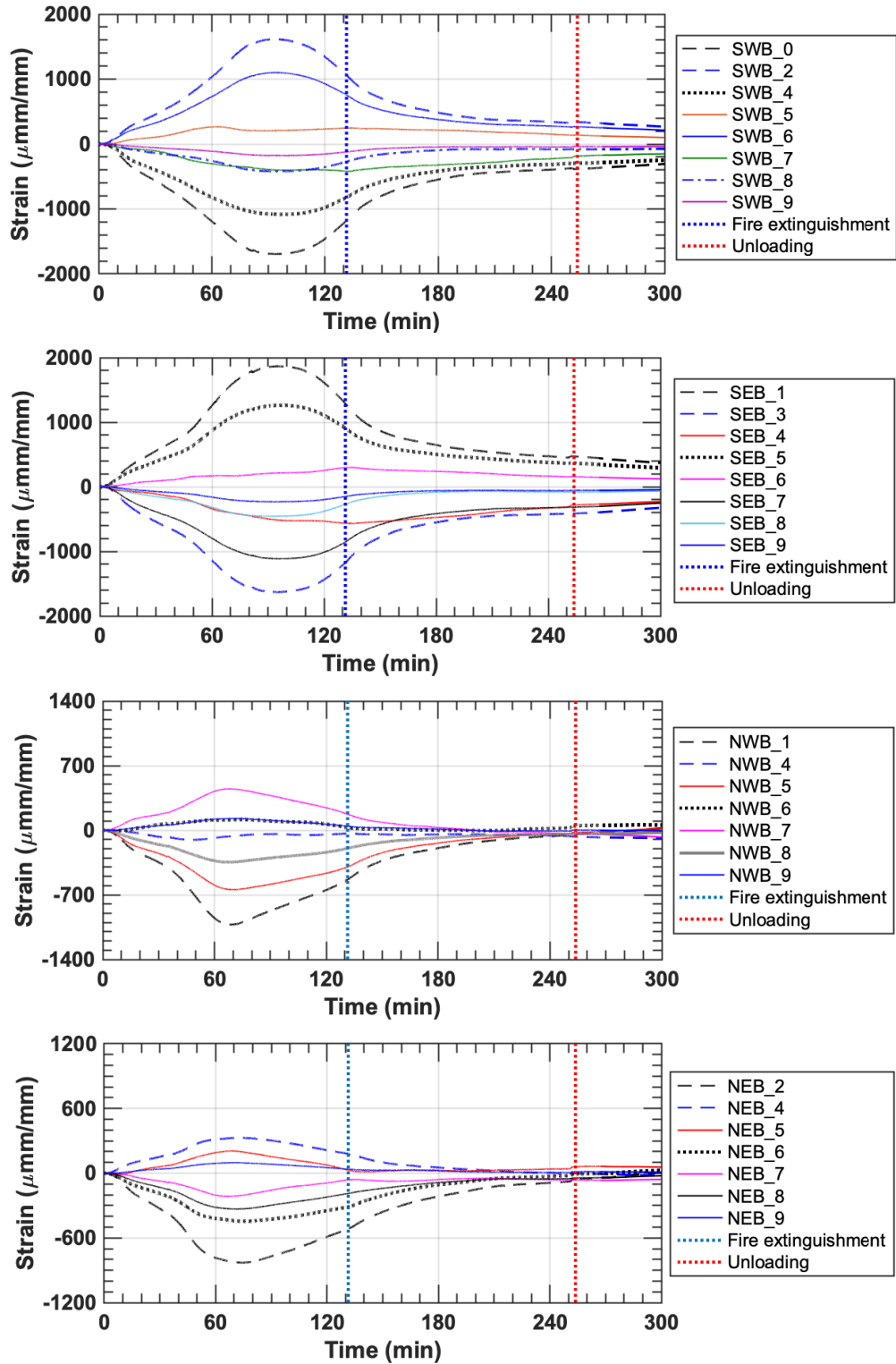
Fig. 65. Strains of test bay columns.
