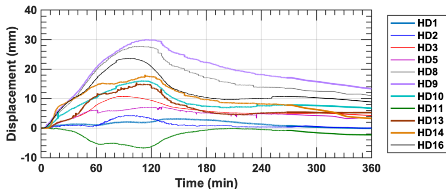
Fig. 32. Measured lateral displacements of the exterior columns.
